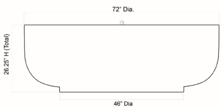
Girona Fountain - 6 Foot (AS) GFRFCFT-1102 627 lbs 72.00"W x 26.25"H
