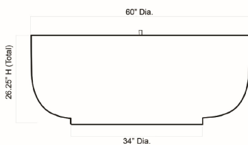
Girona Fountain - 5 Foot (AS) GFRFCFT-1103 464 lbs 60.00"W x 26.25"H
